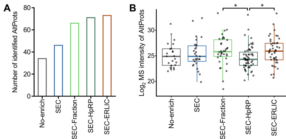
FIG. 4. The effect of fractionation methods on AltProt discovery. The number of identified AltProts (A) and MS intensity of AltProts (B) before and after fractionation. * indicates p < 0.05 for comparison. AltProts, alternative Proteins; MS, mass spectrometry; SEC, size-exclusion chromatography; SEC-fraction, SEC enrichment into 4 fractions; SEC-ERLIC, SEC enrichment followed by ERLIC fractionation; SEC-HpRP, SEC enrichment followed by HpRP fractionation.
