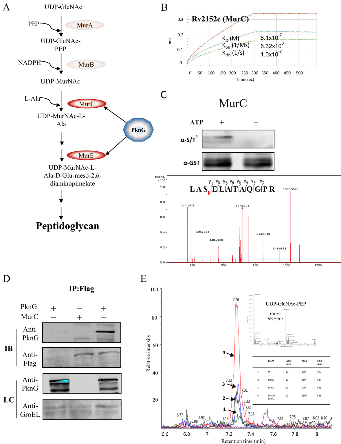
FIG. 6. PknG regulates MurC enzyme activity through interaction with MurC in vivo. A, Schematic of the PG formation with the Mur enzymes. B, In vitro validation of PknG and MurC interaction by BLI. C, In vitro phosphorylation of MurC by PknG. The purified of MurC and PknG were mix with 2:1 in the kinase buffer (50 mM Tris.HCl, 5 mM MgCl 2 , 2 mM MnCl 2 , 1 mM DTT, 5 mM ATP) and incubated in 37 °C for 2 h. D, In vivo validation of PknG and MurC interaction. Flag tagged MurC and PknG were expressed in Msm with ATc induction, PknG interacted with MurC were then immuno-precipitated using an anti-Flag antibody. Anti-PknG and GroEL antibody were loading control. E, MurC activity was enhanced by PknG. MurC activity assay was performed using UDP-GlcNAc, PEP and L-Ala as substrates. The major product of this reaction, UDP-MurNAc-L-Ala, was measured by ultra-performance liquid chromatography coupled with mass spectrometry.
