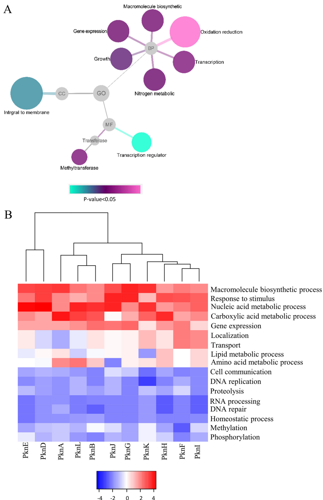
FIG. 2. The STPK binding proteins are functionally diversified. A, Gene ontology (GO) analysis of all the STPK binding proteins. The results were visualized by Cytoscape with p value < 0.05 . B, STPK classification based on functional diversity. The STPKs-KPIs database were analyzed with STRING through Biological Process, and the heatmap was drawn with R language.
